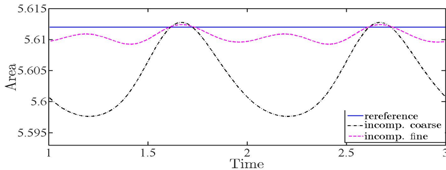
Figure 6: The plot demonstrates the improvement in the area conservation by the finite element incompressible model if the mesh is refined.
