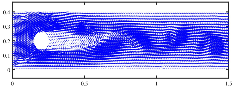
Figure 2: The velocity vector field of the periodic solution at t = 8 .
