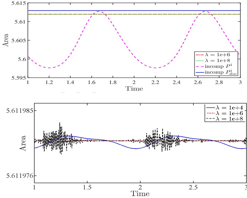
Figure 5: Both plots show the evolution of the area of \Omega_s for different models of vessels wall: neo-Hookean compressible and neo-Hookean incompressible. The bottom plot excludes the incompressible case and shows the area evolution for the other models in a different scale.
