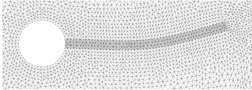
Figure 1: Deformed (virtual) mesh at t = 7.96 , corresponding to the largest displacement in a cross-flow direction. A part of the domain close to the cylinder and the beam is shown.
