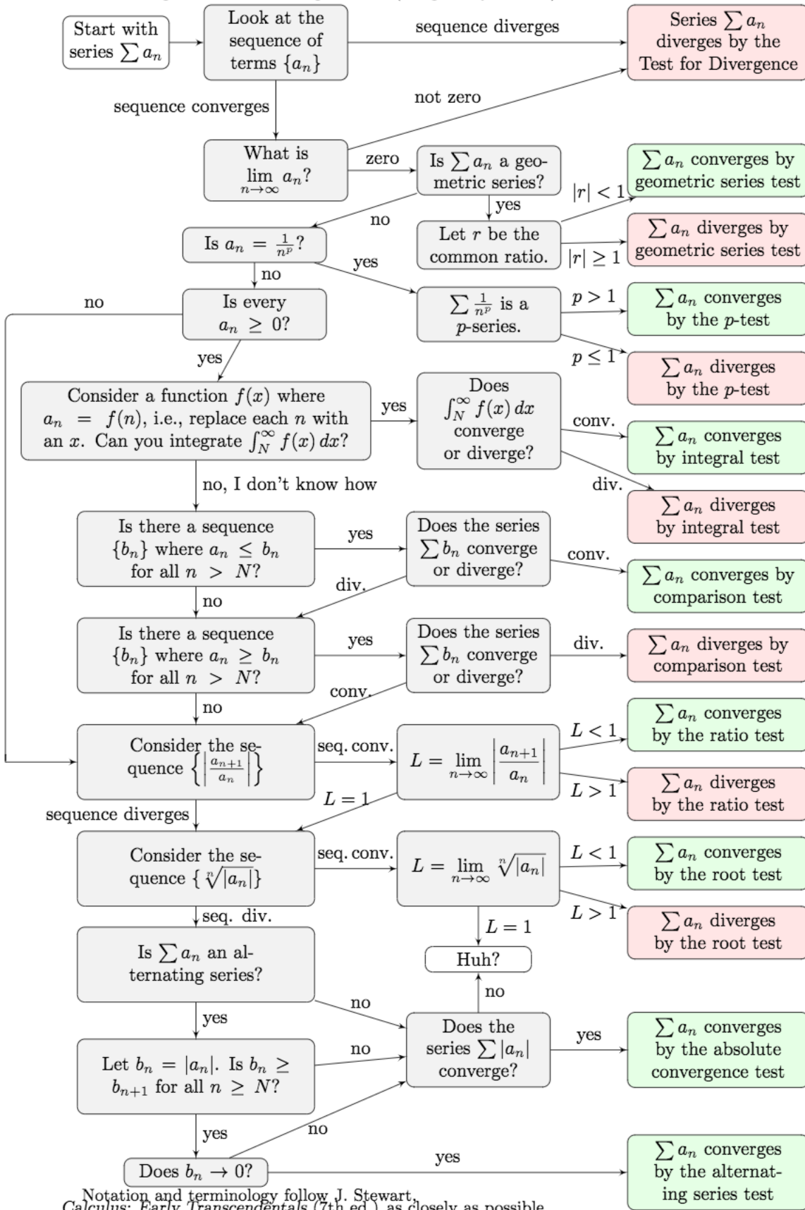
Flowchart summarizing most series convergence test (designed by E. Kim)
